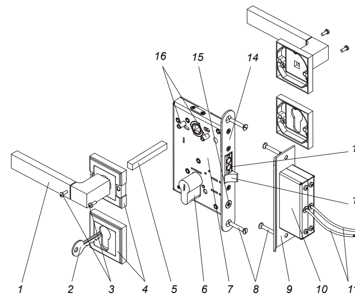
Fig.1. LB-72.4 electromechanical lock design
