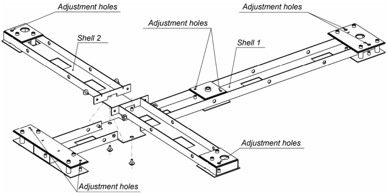
Figure 2. Assembly scheme.
