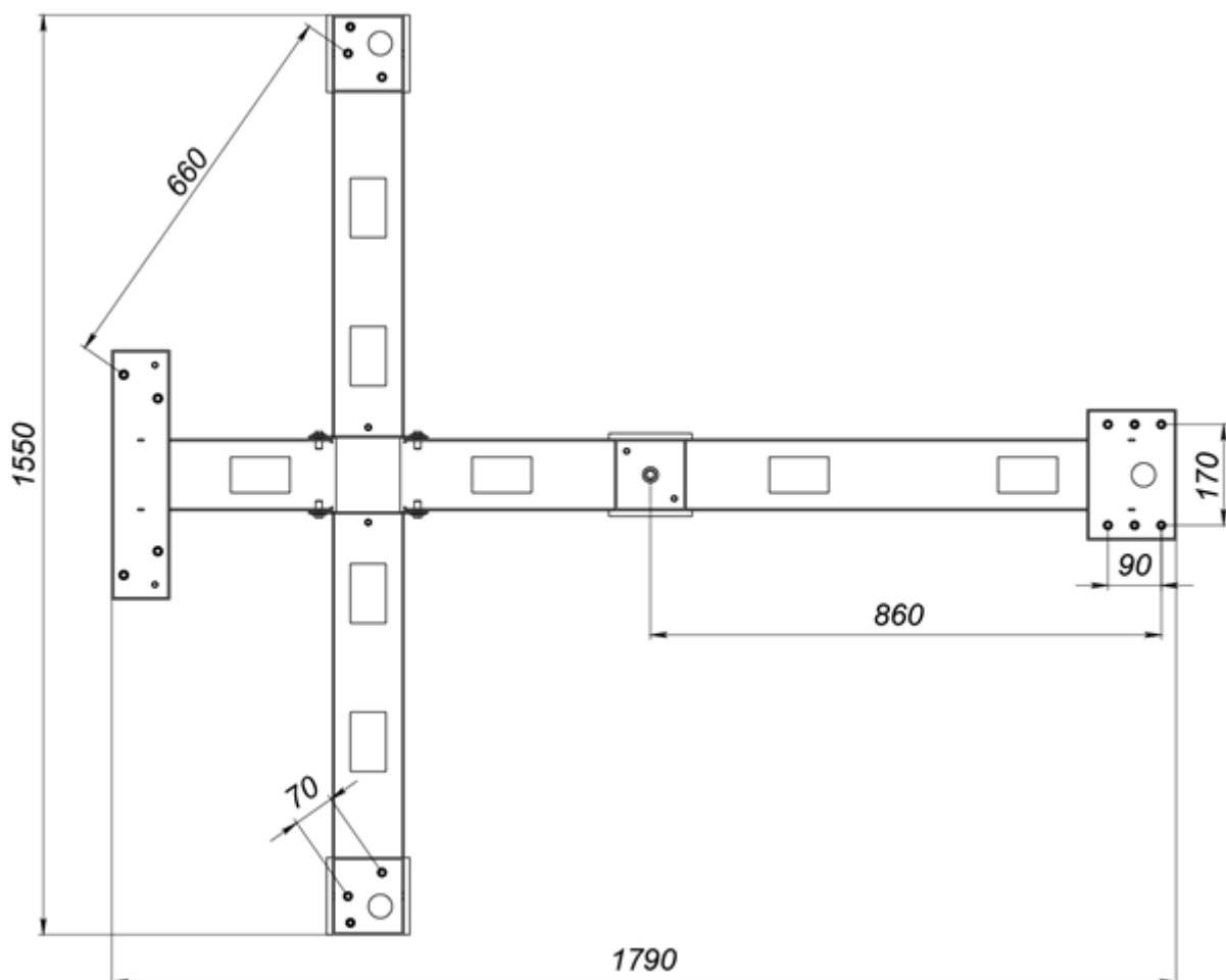
Figure 1. Overall and installation dimensions of the frame
