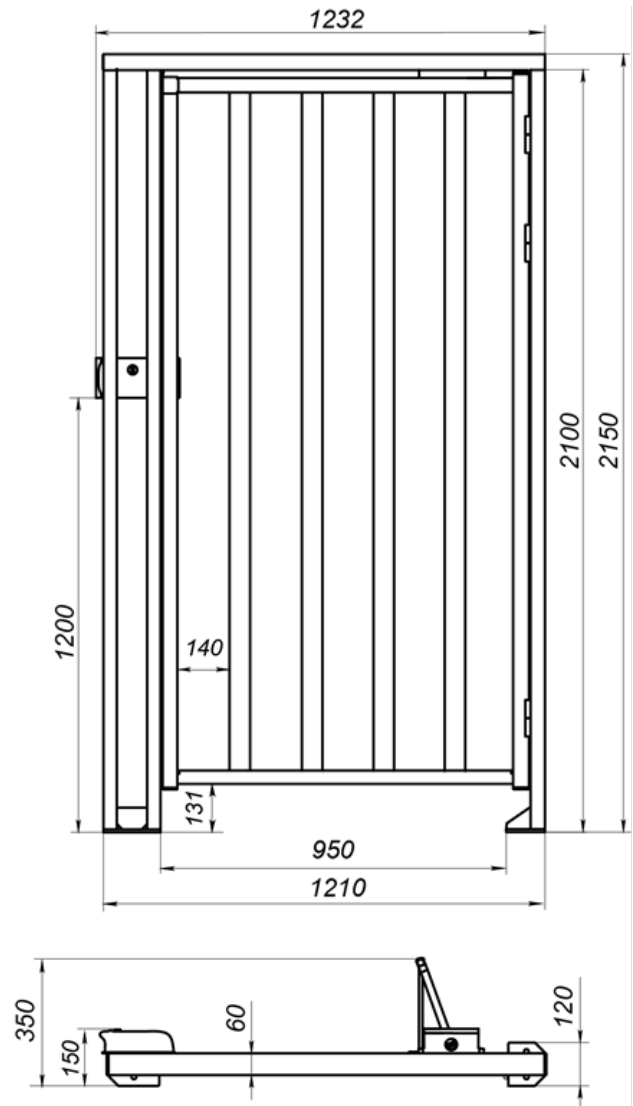
Fig. 2. Overall dimensions of the WHD-15
